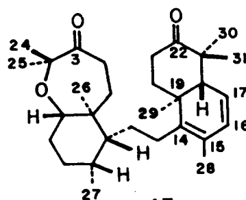
43 Sodwanone C
