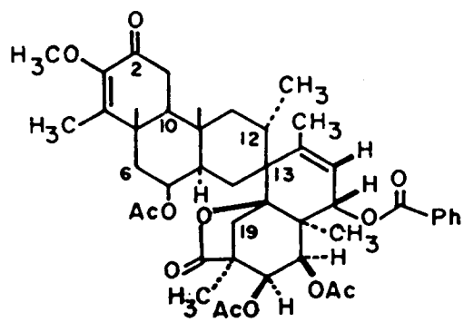
40 Spirocaracolitone
