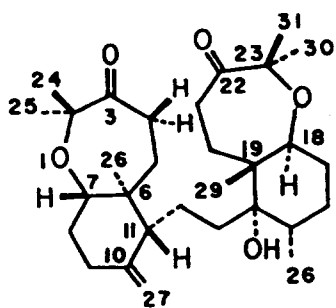
44 Sodwanone D
