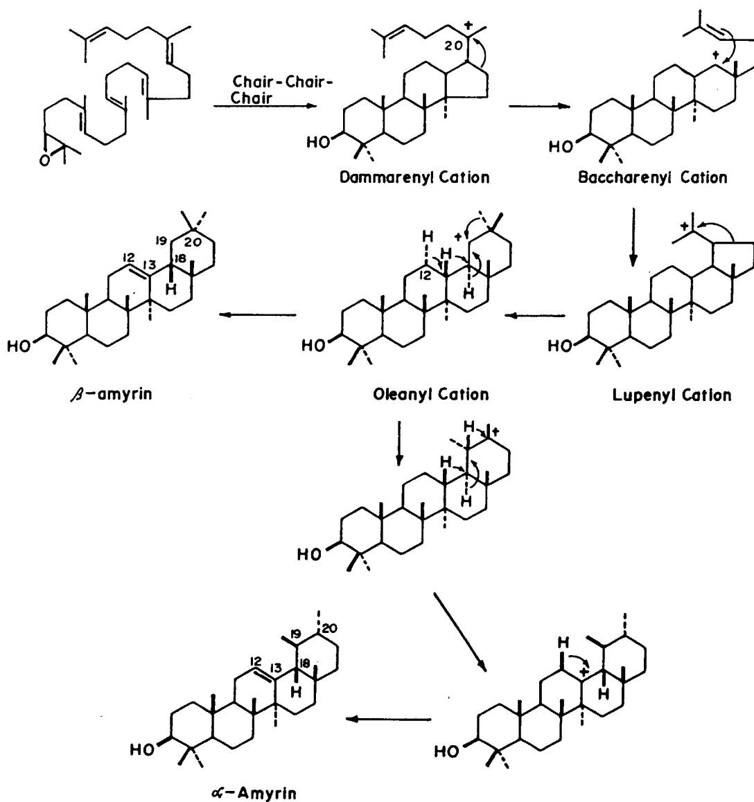
Scheme 1.
