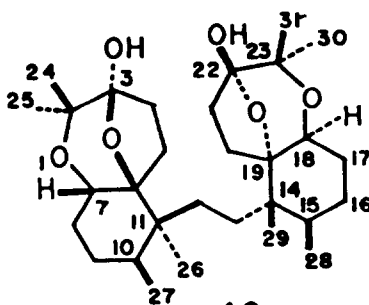
46 Sodwanone F
