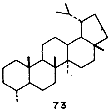
24-Norlupane
