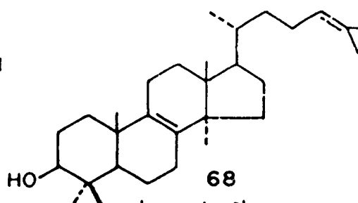
Lanosterol
