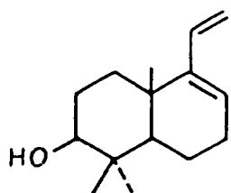
Bicyclic diene
